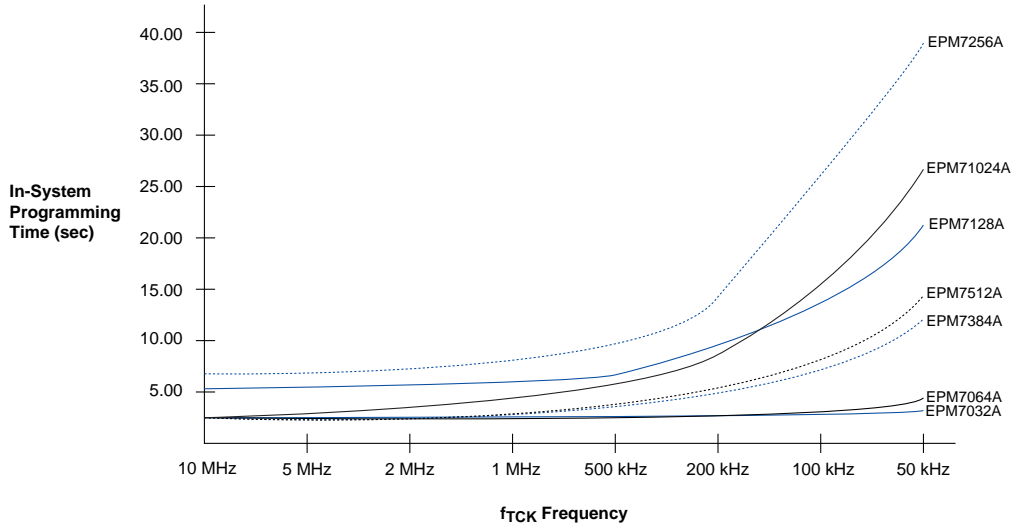
Figure 2. MAX 7000A In-System Programming Times vs. f_{TCK}
