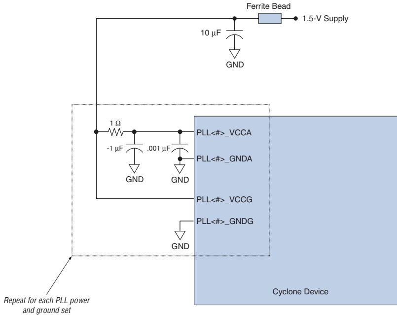
Figure 8. PLL Power Schematic for Cyclone PLLs
