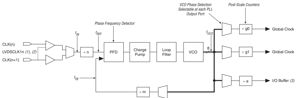
Figure 1. Cyclone PLL
