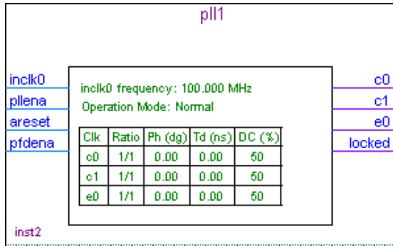
Figure 9. altpll Megafunction Symbol Targeted for Cyclone FPGAs
