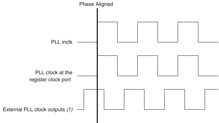
Figure 4. Phase Relationship Between PLL Clocks in Normal Mode
