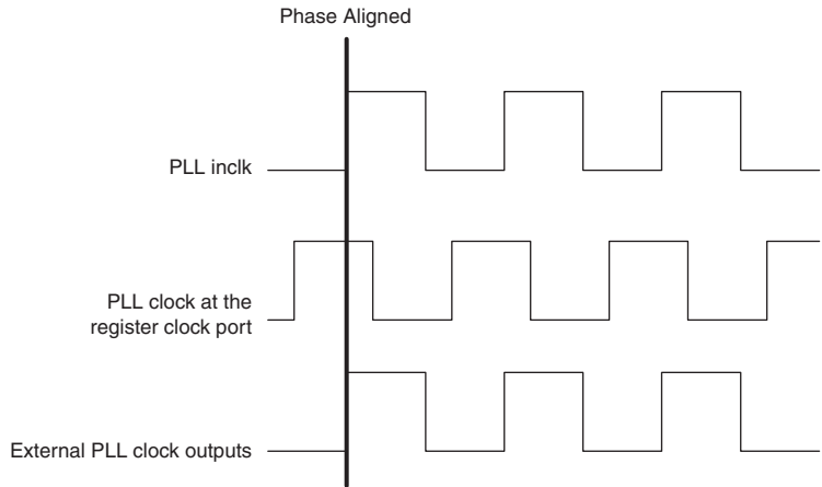
Figure 5. Phase Relationship Between PLL Clocks in Zero Delay Buffer Mode
