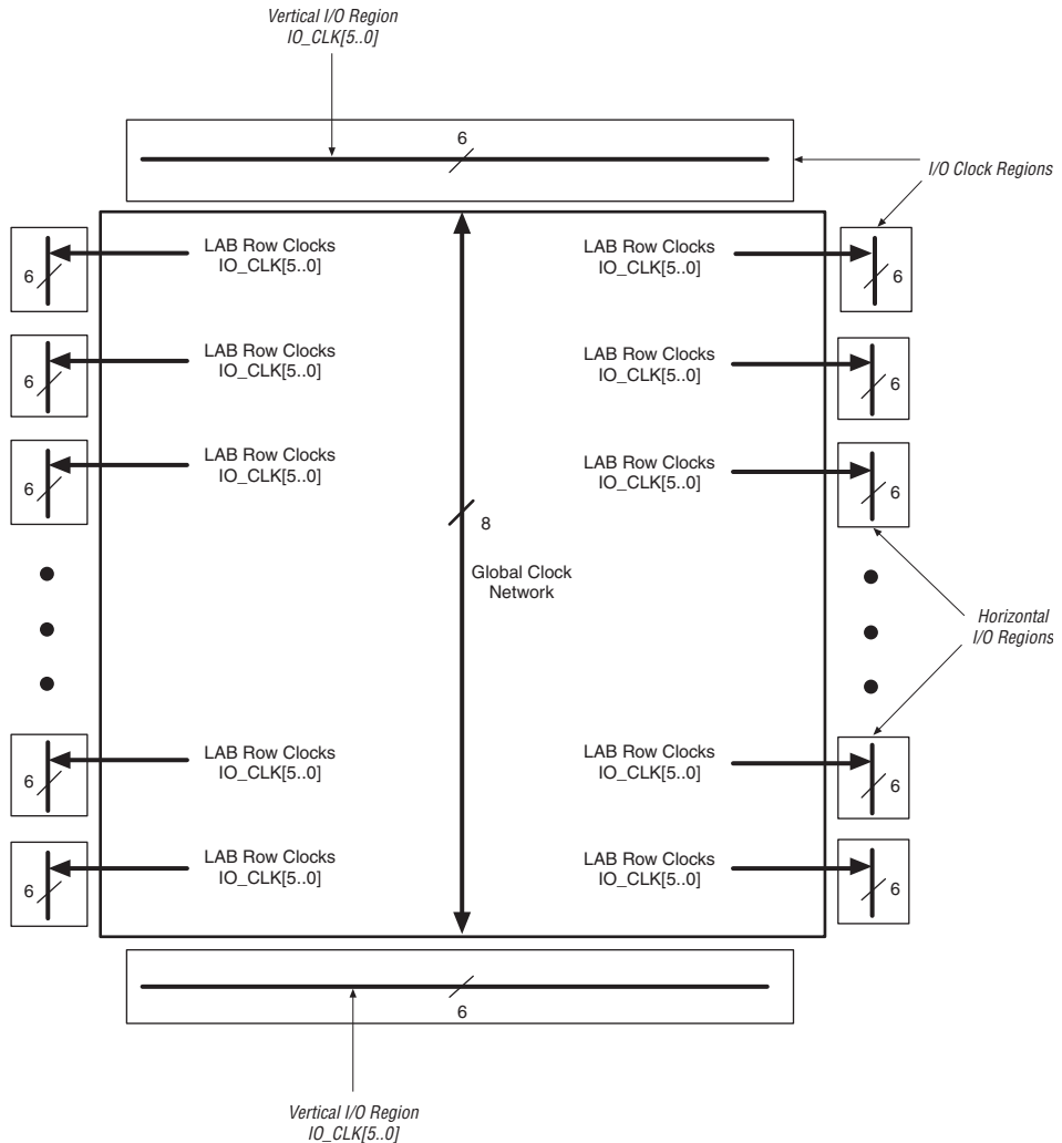
Figure 20. I/O Clock Regions
