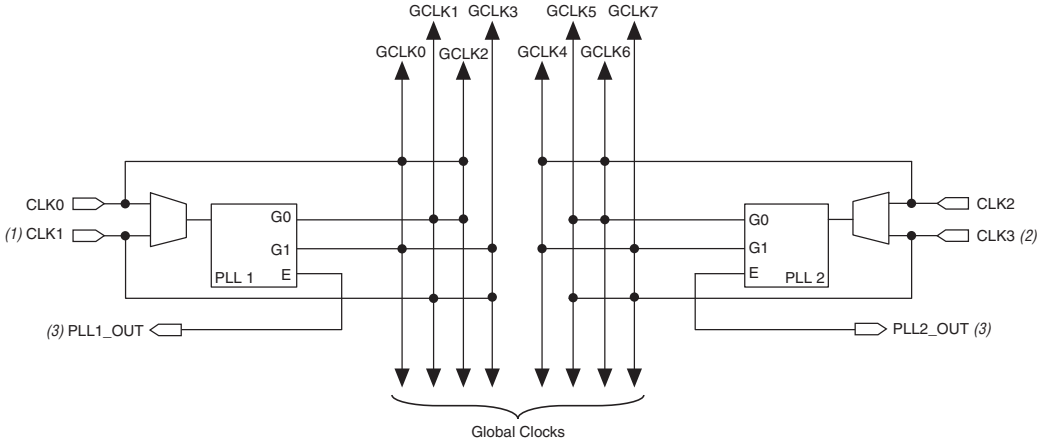
Figure 3. Cyclone PLL Clock Connections
