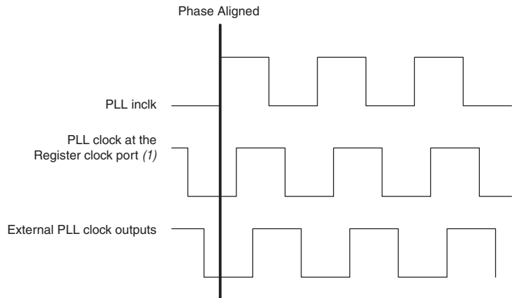
Figure 6. Phase Relationship Between PLL Clocks in No Compensation Mode
