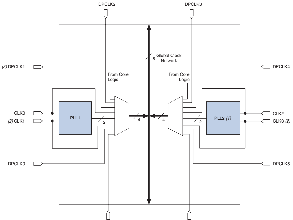
Figure 18. Global Clock Generation
