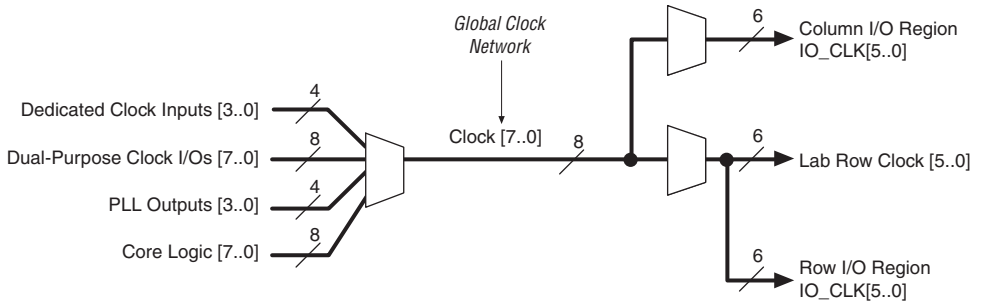
Figure 19. Global Clock Network Multiplexers
