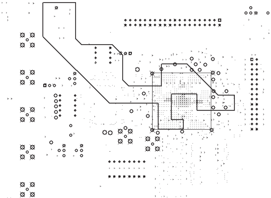
Figure 7. V_{CCINT} Plane Partitioned for V_{CCA} Island
